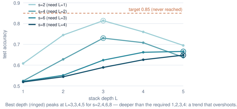
Figure 4: Emergent depth grows with the required receptive field but overshoots it. Under a fair mean over restarts, accuracy is near chance for stacks too shallow to span the spike pair and rises with depth, the optimum deepening with s ; but it never reaches the 0.85 target and the best depth exceeds s/2 (the clean target-crossing staircase was a best-of-restarts artifact).
