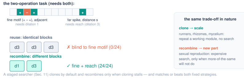
Figure 6: Reuse vs recombination, and the clone/recombine trade-off nature also makes. One reused block suffices for repetitive structure; a task needing two different operations forces recombination of different blocks.
