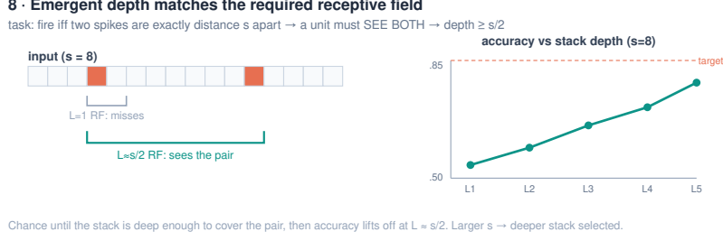
Figure 4: Emergent depth matches the required receptive field. Accuracy is at chance until the stack is deep enough for its receptive field to span the spike pair, then rises sharply at depth \approx s/2 .
