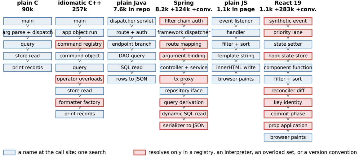
Fig. 1. The path a reading agent resolves through one endpoint of each pair, plain beside layered, with its tokens-to-trace in the header (each pair at one counting granularity). Every red step is an indirection: the name at the call site does not reach the deciding code.
