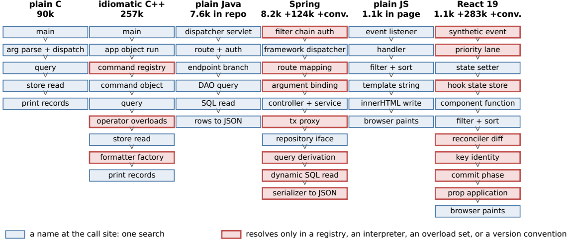
Fig. 1. The path a reading agent resolves through one endpoint of each pair, plain beside layered, with its tokens-to-trace in the header (each pair at one counting granularity). Every red step is an indirection: the name at the call site does not reach the deciding code.
