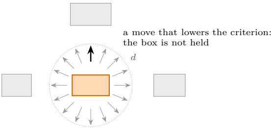
Figure 1 The test, one box and one criterion. The box is moved a distance d , two per cent of the drawing's width, in each of sixteen exact directions, and the criterion is recomputed. If some move lowers it (the dark arrow), the box is not held; if every move raises it, the box is held .
