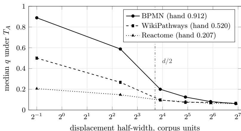
Figure 4: What the half-grid jitter test can and cannot see. T_A has its corner at agreement, so a box offset by \epsilon is released only when a move of radius d lowers the term, and moving d toward the agreement lands at d - \epsilon : below \epsilon = d/2 nothing changes. Half the detected pitch is 0.5 units, at the left edge, which is why the declared test leaves every corpus where it found it. Past d/2 the hold falls to the grid-snapped level of 0.06 to 0.08.
