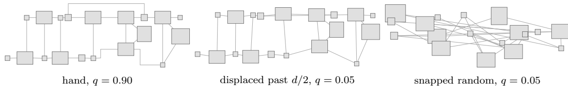
Figure 4: The grid alternative of Section 7: the grid alone does not produce the alignment hold. One BPMN model, 19 boxes; the corpus medians are 0.91, 0.20 and 0.07. Left, the drawing as its author left it. Centre, every box displaced by up to 15 units, just past the d/2 below which the directional test cannot resolve a misalignment. Right, every box placed uniformly at random in the same bounding box and snapped to the same grid: the grid is available and the author is not. Box sizes are unchanged throughout. The hand panel draws the routes the file stores; the two control panels draw chords, their boxes no longer being where the routes ran.
