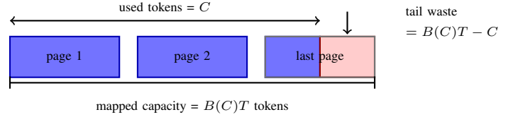
Fig. 1: Tail waste under paged KV allocation. A request with context length C maps B(C) = \lceil C/T \rceil pages, each holding T tokens, so the unused capacity in the final mapped page is B(C)T - C .
