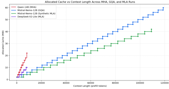
Fig. 2: Allocated cache versus context length across the four measured runs. MHA and DeepSeek grow faster in allocated cache than the two Mistral variants, while the synthetic MLA conversion yields the smallest long-context growth among the Mistral pair.
