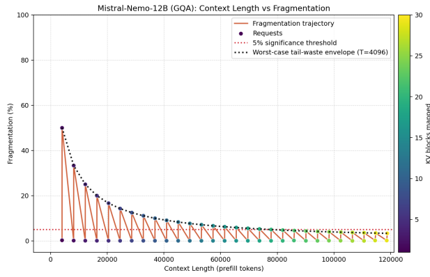
(a) Measured Mistral-Nemo-12B GQA fragmentation with a worst-case analytical envelope.
