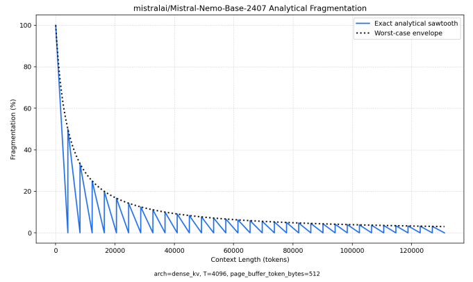
(b) Exact analytical sawtooth for the same geometry.
