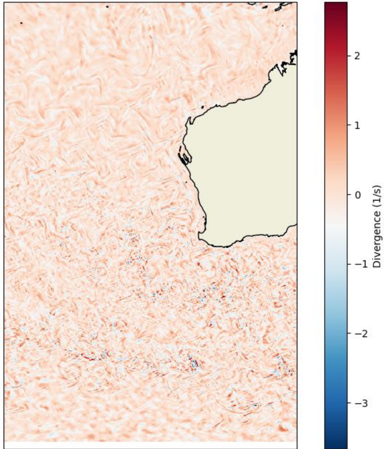
Surface Ocean Current Divergence - Western Australia 1e-5
