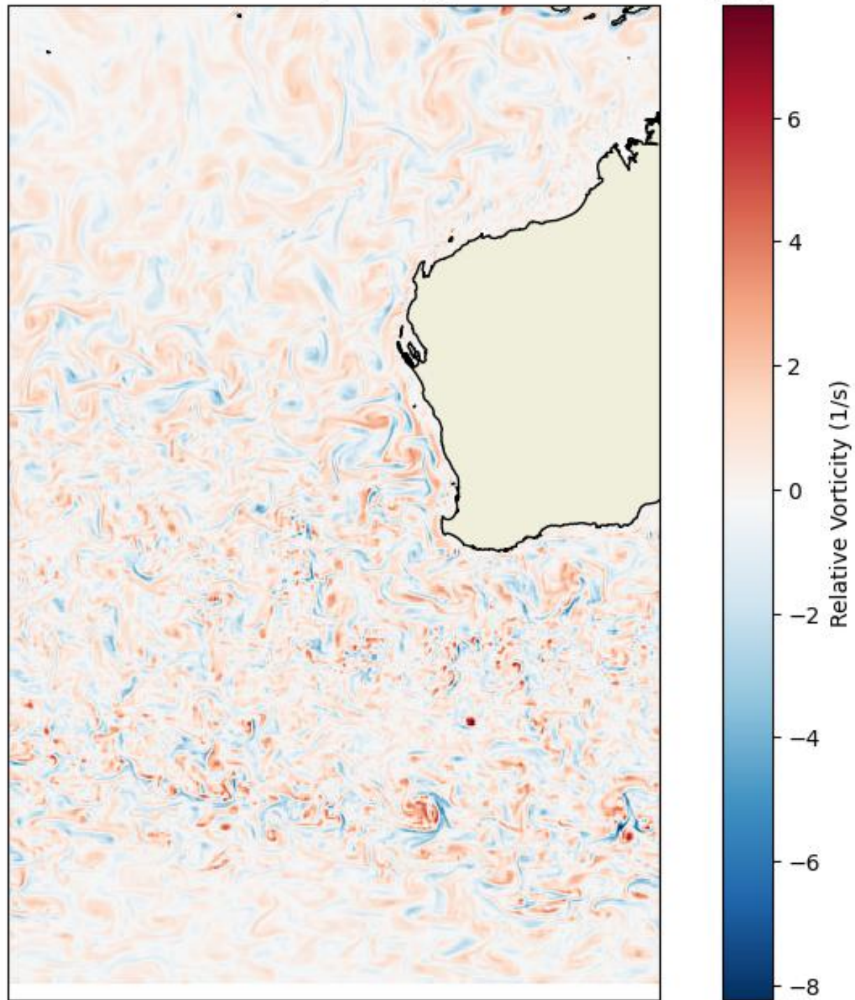
Surface Ocean Current Curl (Vorticity) - Western Australia 10^{-6}
