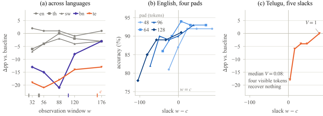
Figure 2: Three sweeps of the same mechanism, each paired against its own uncompressed baseline. (a) Five languages against the window; ticks below the axis mark each language’s c , and the two languages whose trailing block exceeds most tested windows are drawn in colour. (b) English, four instruction pads, against the slack w - c : the conditions collapse onto one curve and the rule at w=c separates every cell at most 90% from every cell at least 91%. (c) Telugu, same x -axis as (b): English is at its ceiling within about ten tokens of slack, Telugu needs eighty.
