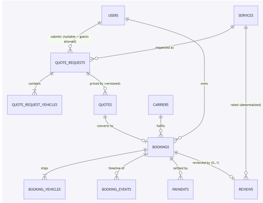
Figure 3.1: Entity relationships across the core transaction flow.
