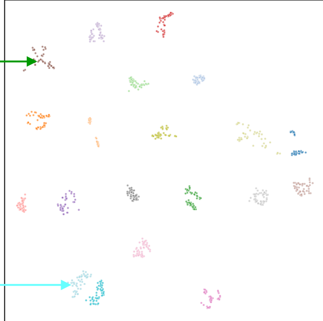
Task Cluster
