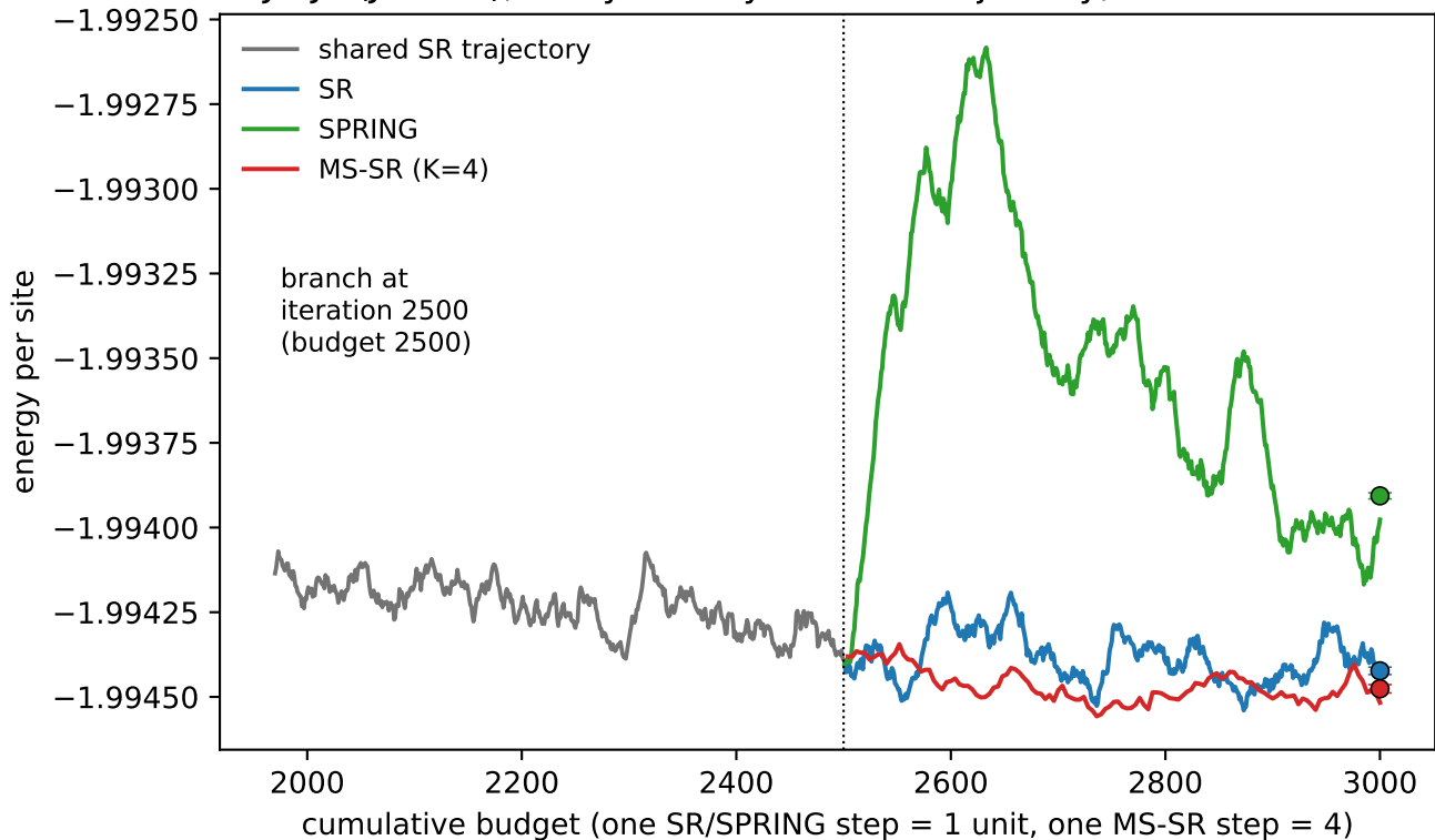
8x8 J1-J2 ( J_2=0.5 ), no-symmetry ViT: one trajectory, three continuations
