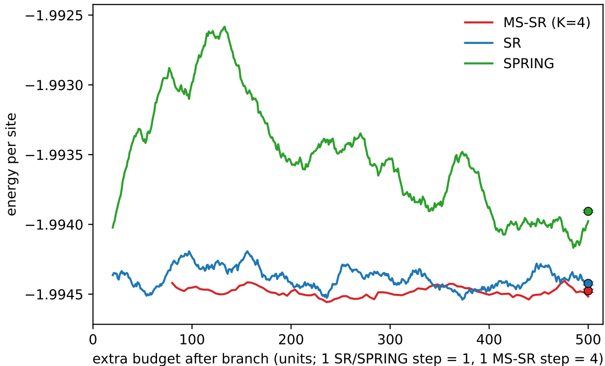
8x8 J1-J2 ( J_2=0.5 ): branch at iteration 2500, equal extra budget
