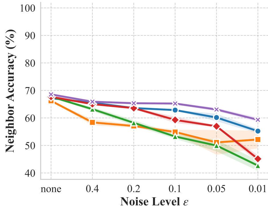
CIFAR 100 ( N=25 )
