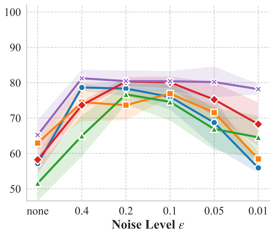
Food 101
