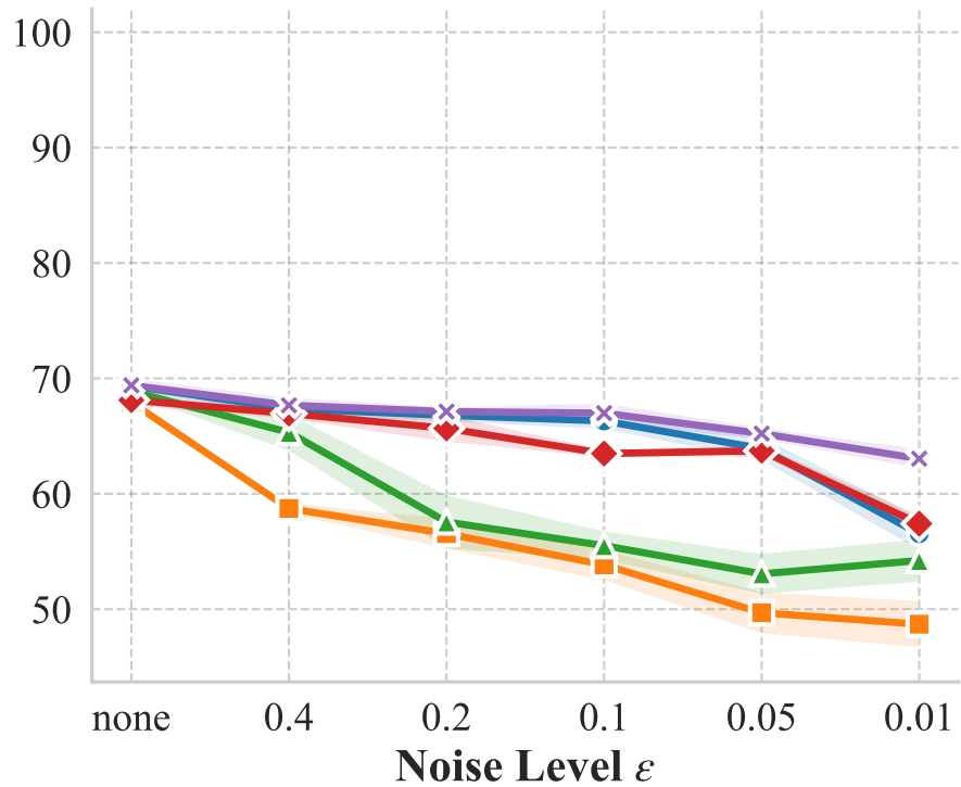
CIFAR 100 ( N=50 )
