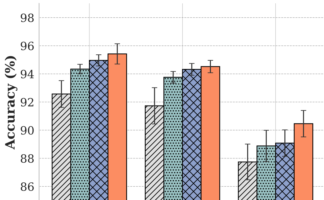
Stanford Dogs - Local Accuracy
