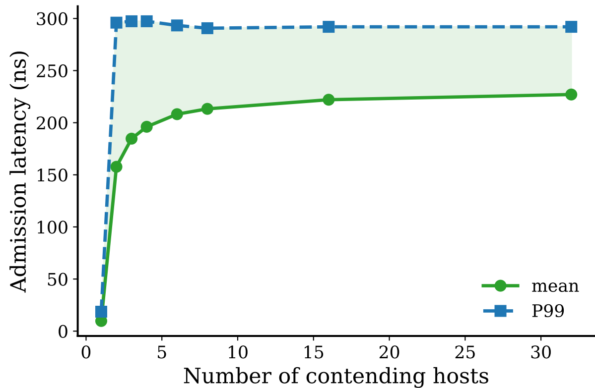
Per-VC arbitration bounds multi-host admission tail
