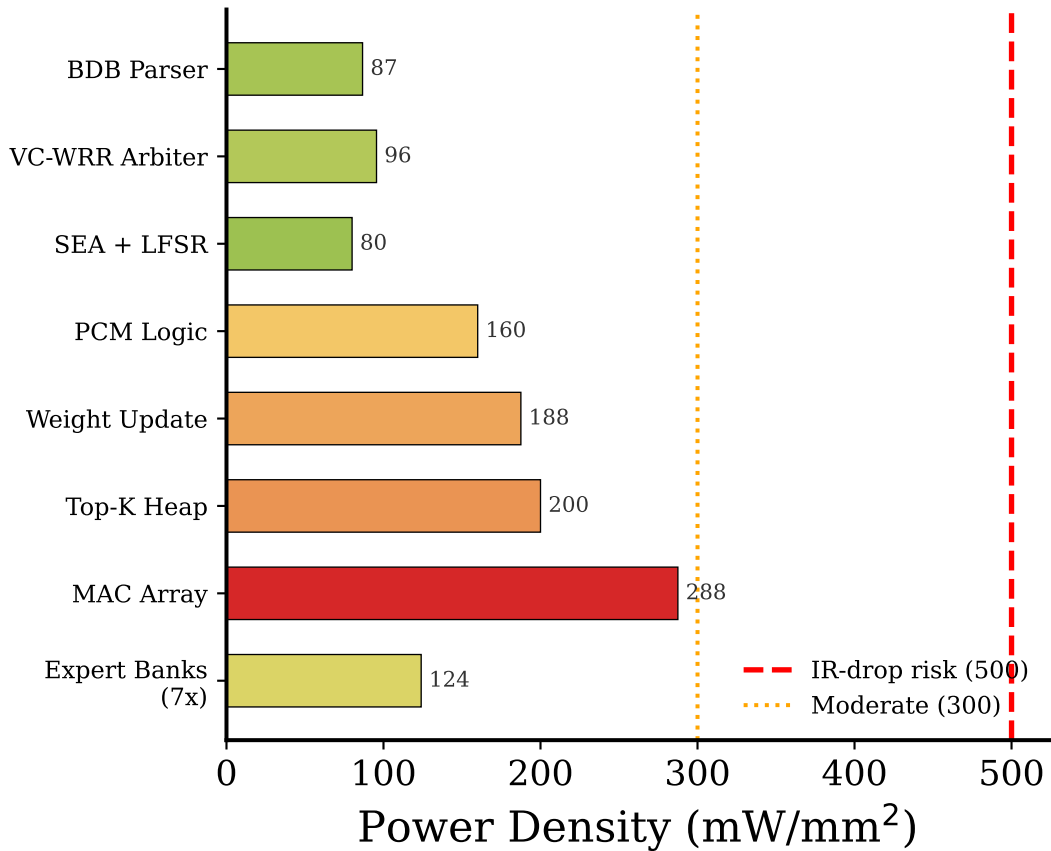
(b) Per-Block IR-Drop Risk
