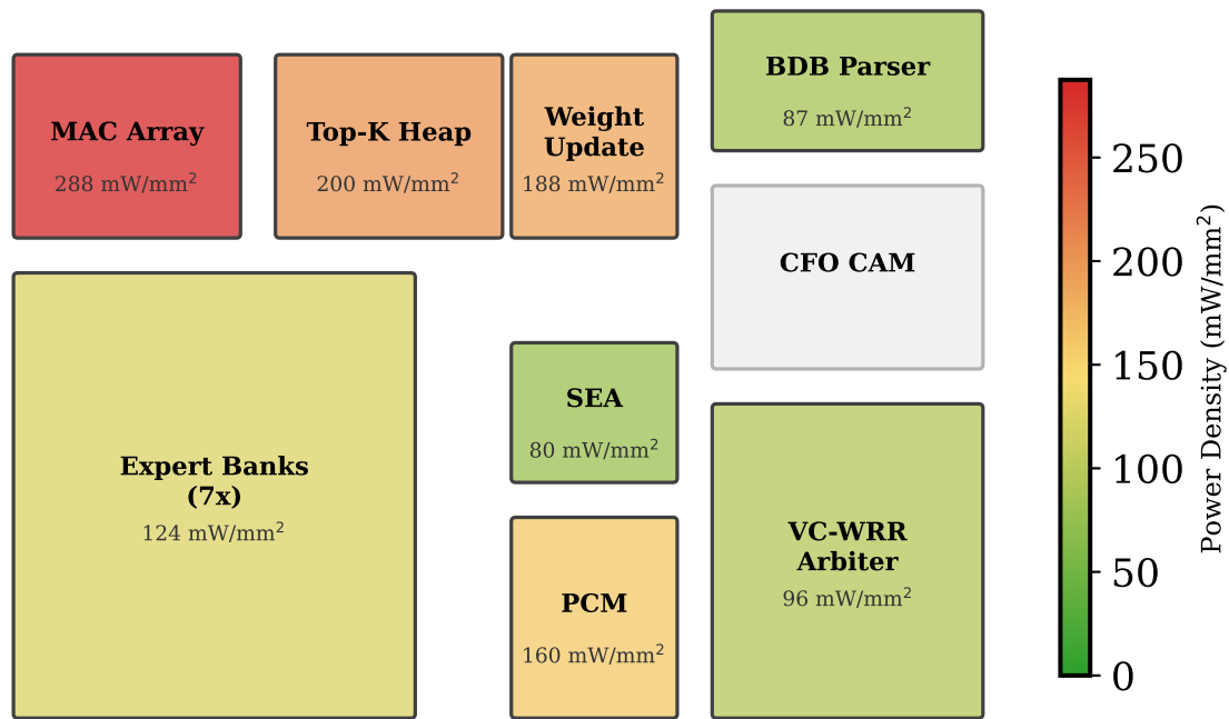
(a) Power Density Floorplan (ASAP7 7nm, 1 GHz)
