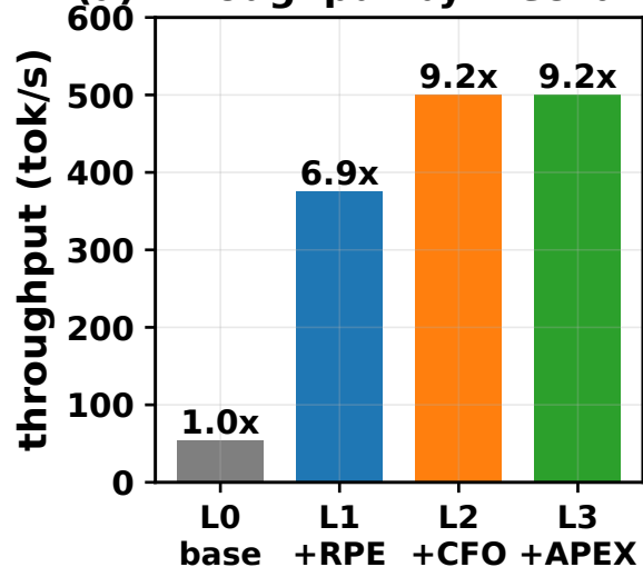
(a) throughput by mechanism
