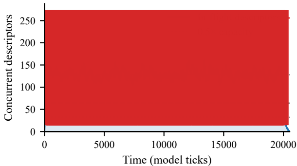
Capacity 64 chunks
