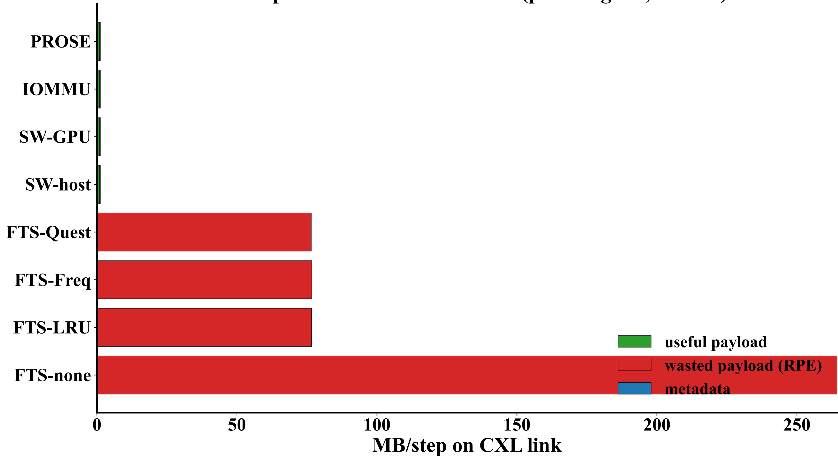
Per-step CXL traffic breakdown (pathological, 4 GB/s)
