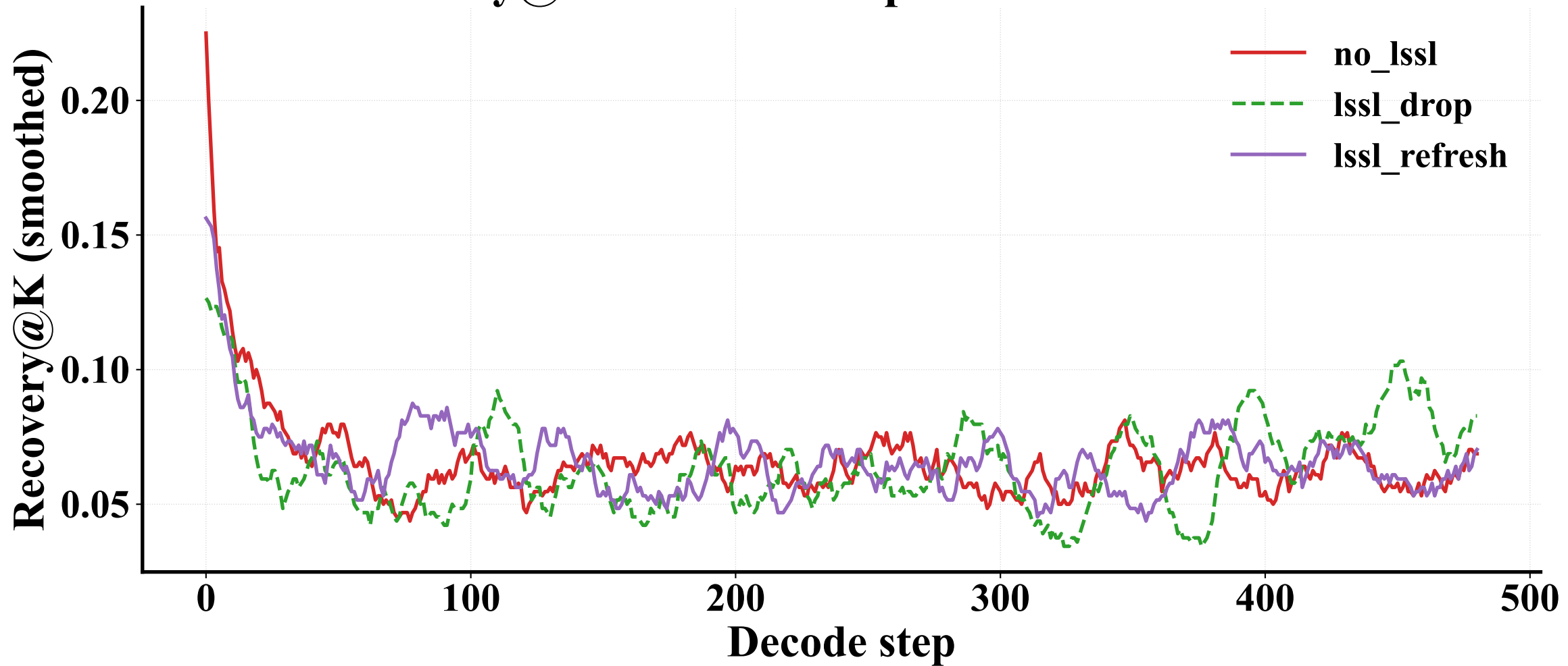
Recovery@K trace under speculative-decode drift
