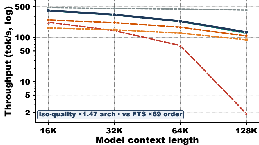
(b) Decode throughput
