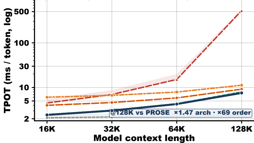
(a) TPOT (P50 line, P99 band)
