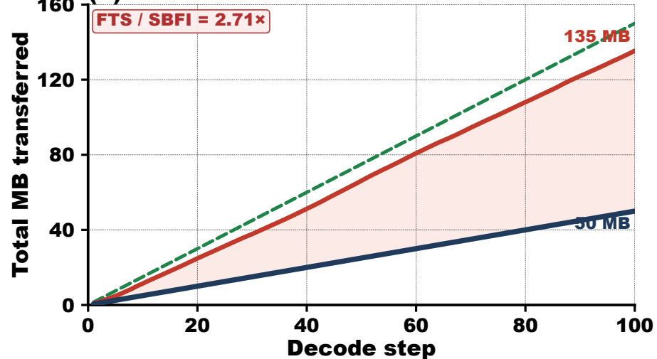
(b) Cumulative CXL traffic
