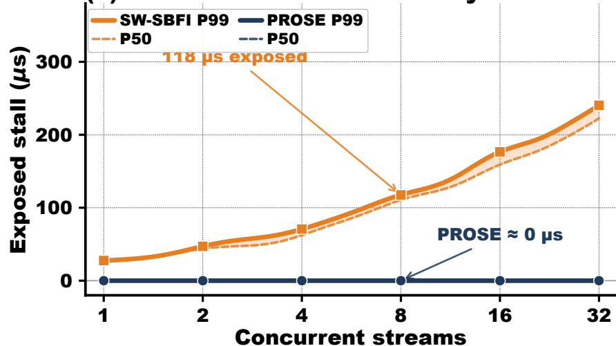
(c) Tail stall under concurrency
