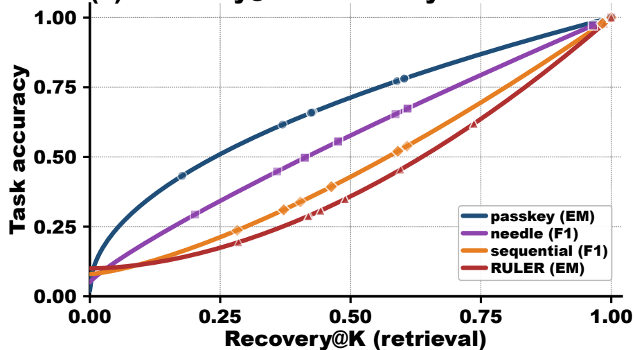
(c) Recovery@K → accuracy calibration
