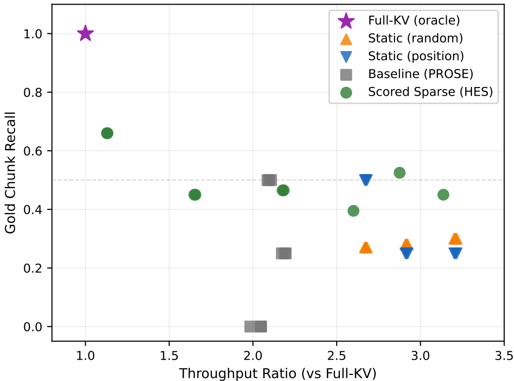
Recall-Throughput Pareto: Scored vs Unscored Enforcement
