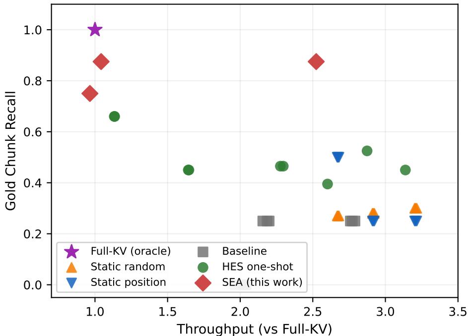
Recall-Throughput Pareto: Scored vs Unscored Enforcement
