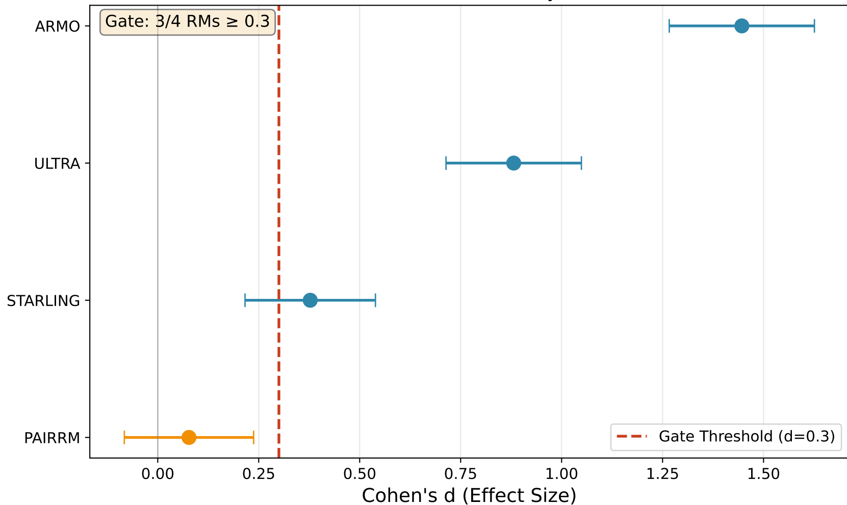
Enumeration Preference Effect Size by Reward Model (Positive = Enumerated > Synthesized)
