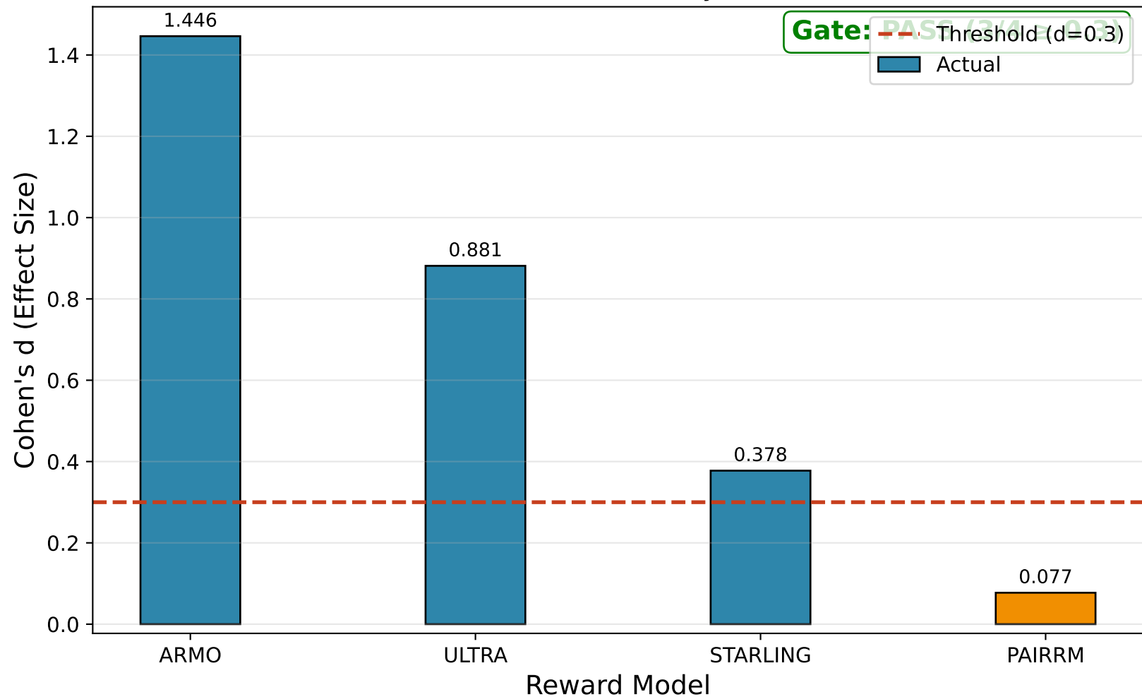
Gate Condition: Effect Size by Reward Model
