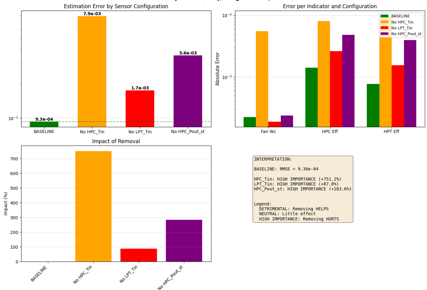
Ablation Study Results (noisy, 1ctx_3sensors | row 53)
