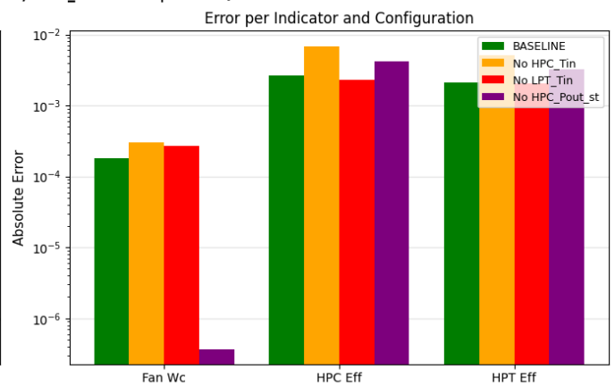
Ablation Study Results (clean, 1ctx_3sensors | row 53)
