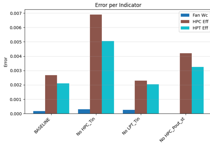
Ablation Study Results (clean, 1ctx_3sensors | row 53)
