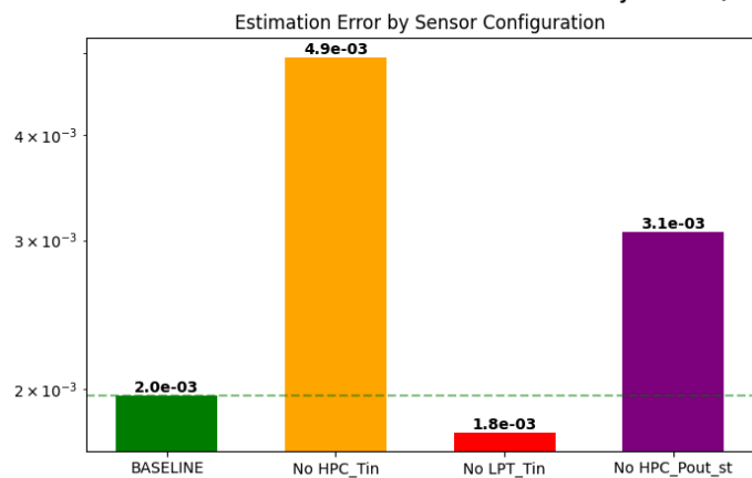
Ablation Study Results (clean, 1ctx_3sensors | row 53)
