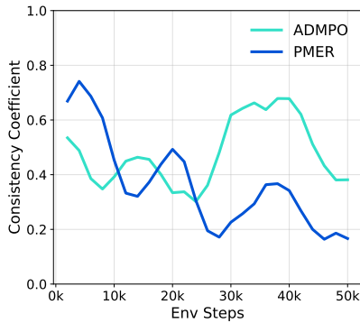
Figure 4: Empirical estimate of L_s^{(k)}(\hat{T}_\phi) on Hopper. We estimate the k=10 consistency coefficient by discretizing the state space into bins, constructing the policy-induced closed-loop transition kernel using the learned dynamics model, computing its k -step kernel P^k , and evaluating \delta(P^k) = \frac{1}{2} \max_{i,j} \|P^k(i, \cdot) - P^k(j, \cdot)\|_1 . Lower values indicate better finite-horizon multi-step consistency.
