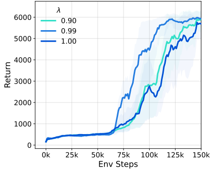
Figure 1: \lambda ablation (Humanoid).
