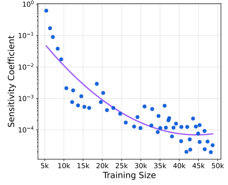
Figure 5: Empirical estimate of \delta_{\hat{T}_\phi} versus training size.
