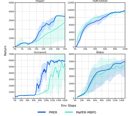
Figure 6: Comparison between PMER and MaPER-MBPO on the four benchmark environments used in MaPER.
