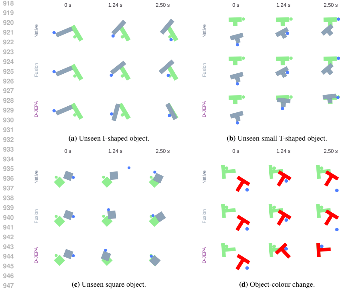
Figure 13: Matched decisions under geometric and visual change. Native selection, calibrated fusion and D-JEPA share the start, goal and candidate pool in every panel. The frames span the complete selected sequence and retain the measured success or failure outcome.
