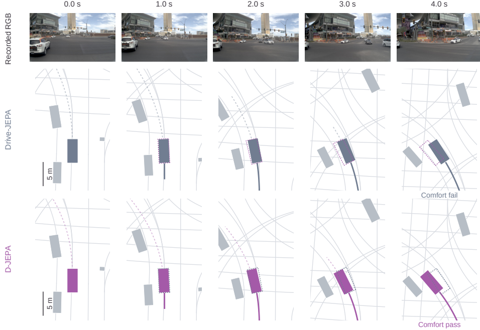
Figure 20: Aligned turning satisfies the comfort criterion. Columns sample the four-second trajectory at one-second intervals. Paired windows follow the mean position; dashed footprints locate the alternative ego position. Only D-JEPA passes the trajectory-level comfort criterion, while both methods pass the recorded collision and TTC criteria.
