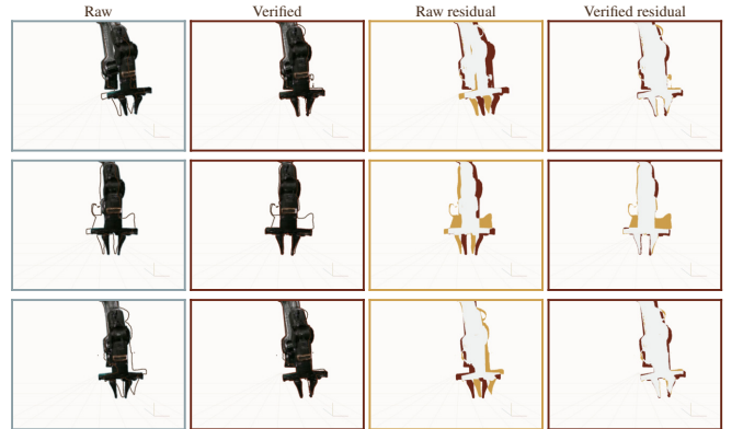
Fig. 12. Real-world PiPER alignment on three matched cases. Columns show measured and verified gripper regions and residuals; gold/brown indicate missed/excess foreground.
