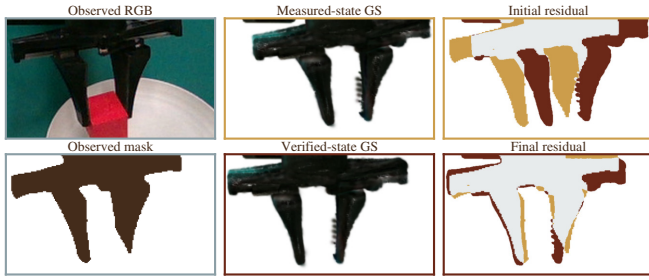
Fig. 13. Saved-state spatial diagnostic workflow. A recorded image and its target mask provide separate visual evidence for evaluating the measured-state render, proposed correction, and verified residual before the synchronized state is committed.
