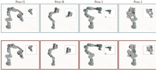
Fig. 6. Controlled Franka recovery on held-out poses G–J. Top: measured state. Bottom: KineSync-GS verified state.
