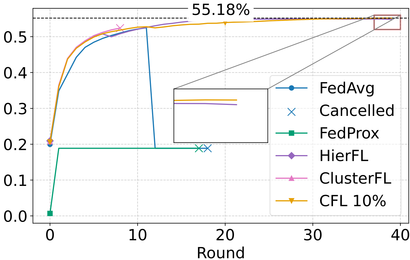
Global Accuracy
