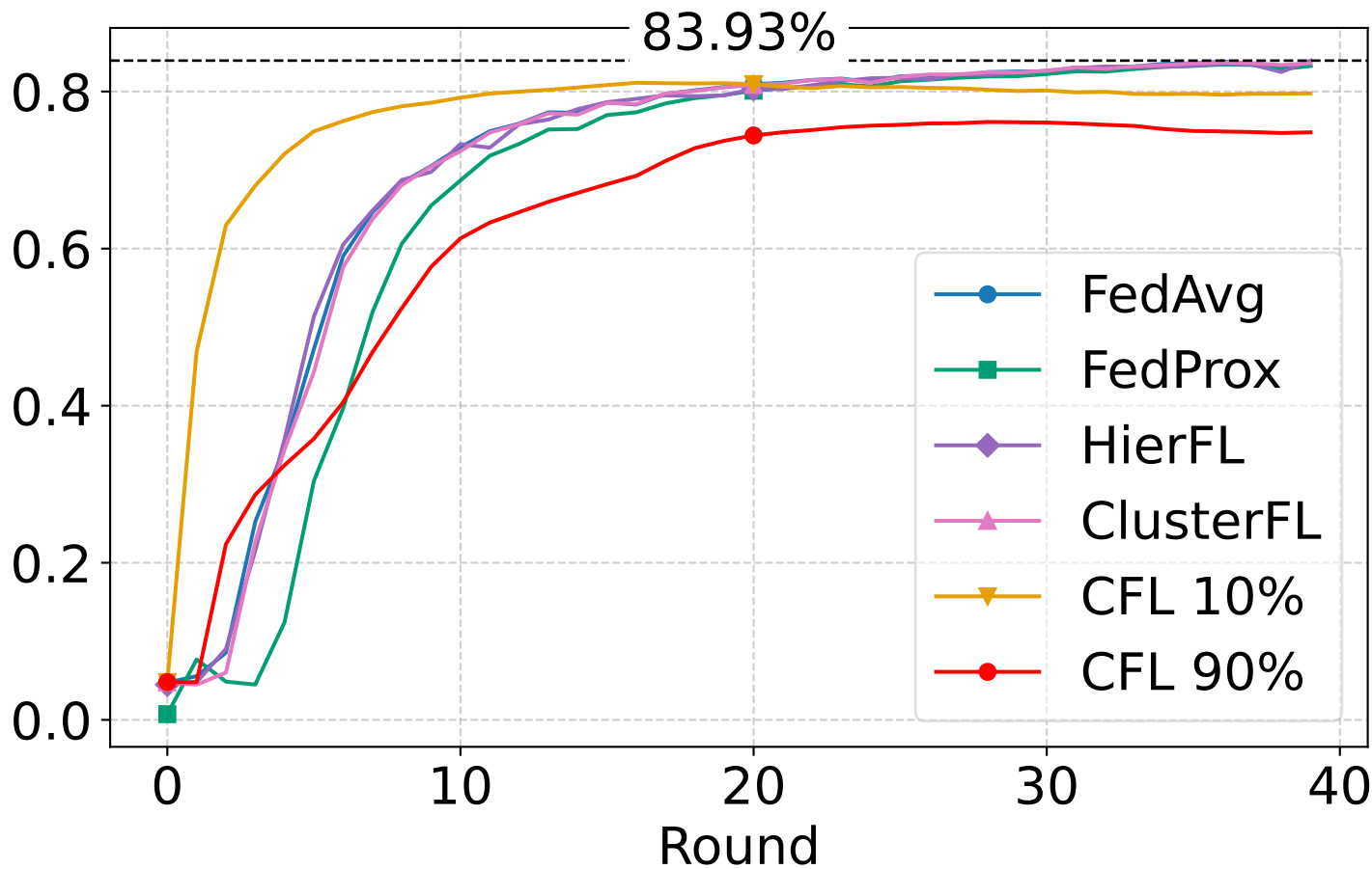
Global Accuracy
