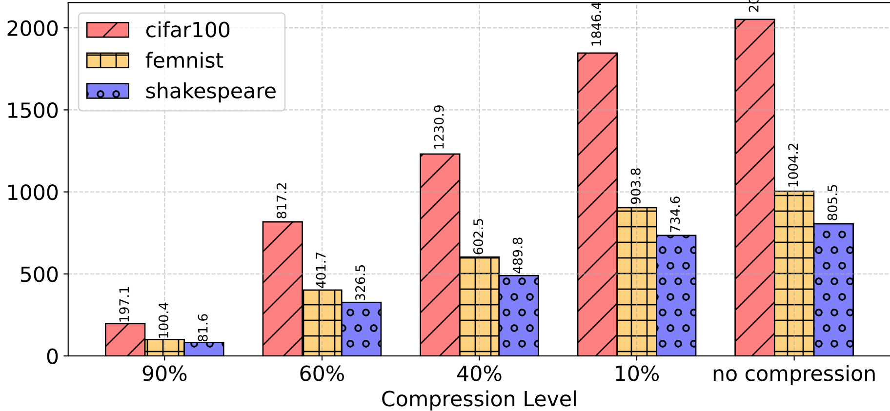
Communication Cost (MB)
