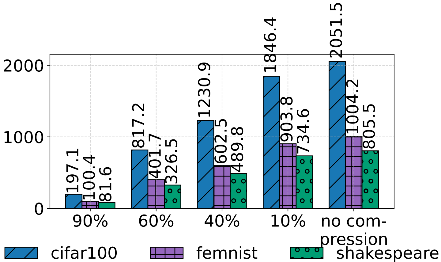
Communication Cost (MB)
