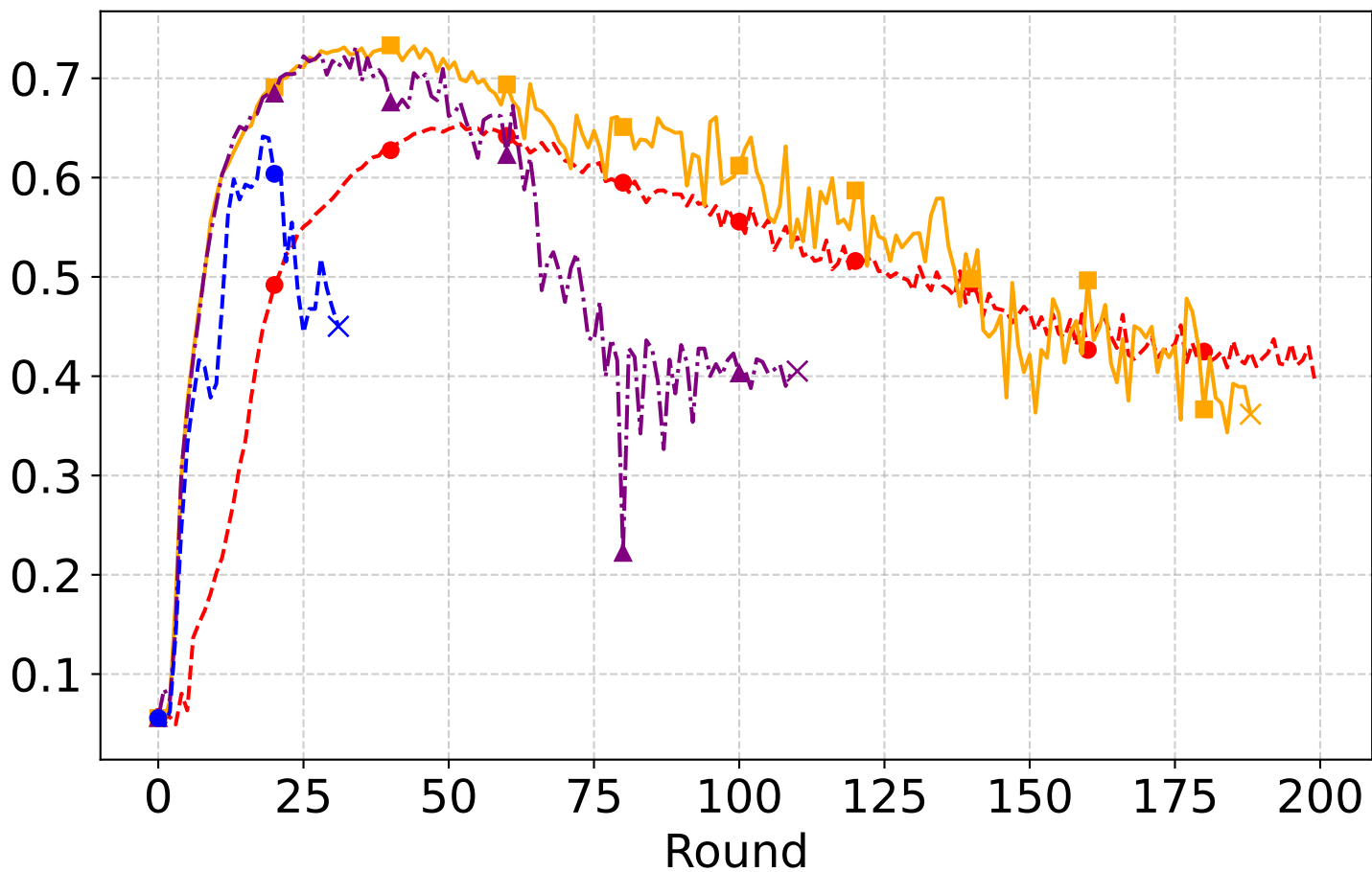
Global Accuracy
