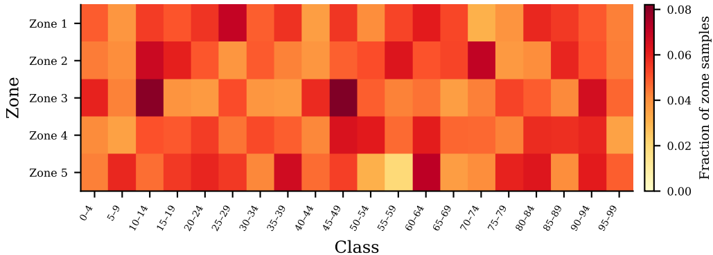
CIFAR-100 — normalised class distribution per zone ( \alpha_{\text{inter}}=5 )
