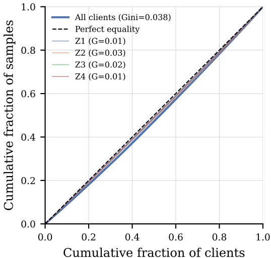
CIFAR-100 — Lorenz curve of client data sizes Overall Gini = 0.038
