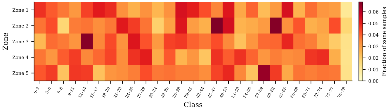
Shakespeare — normalised class distribution per zone ( \alpha_{\text{inter}}=5 )
