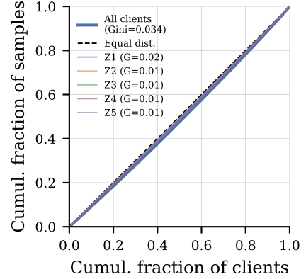
(F) Lorenz curve (Gini=0.034)
