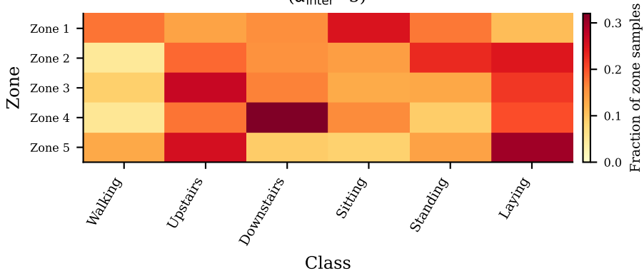
UCI-HAR — normalised class distribution per zone ( \alpha_{\text{inter}}=5 )
