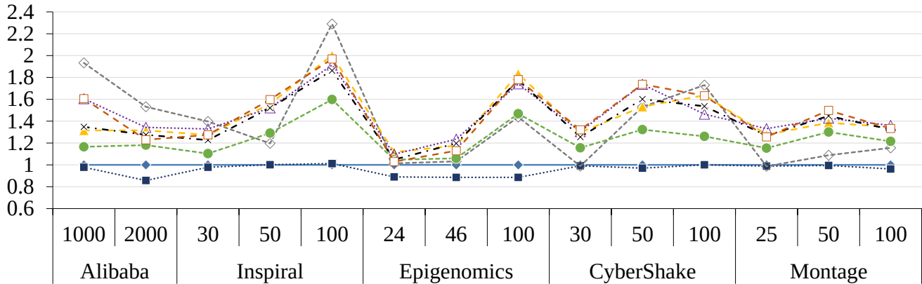
Norm. Makespan
