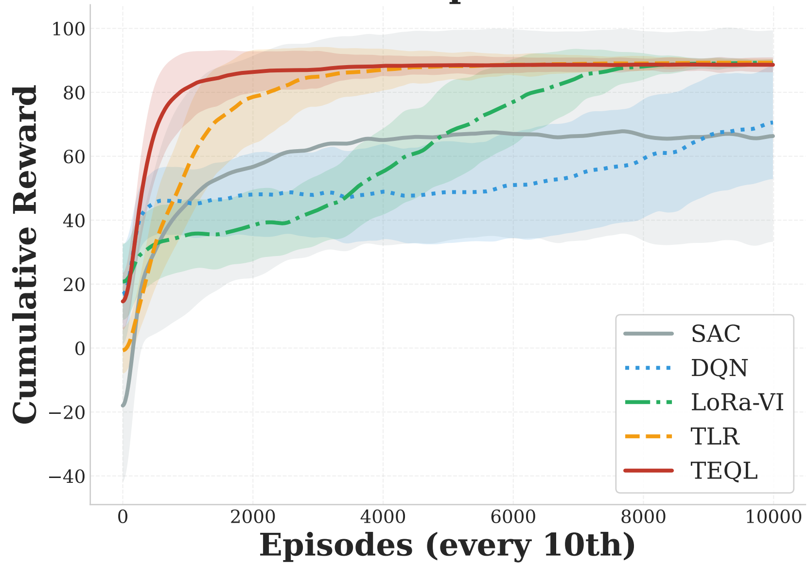
Cartpole
