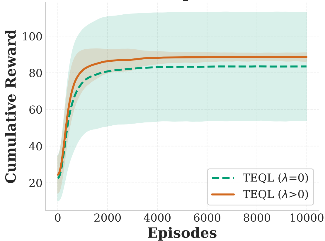
Cartpole
