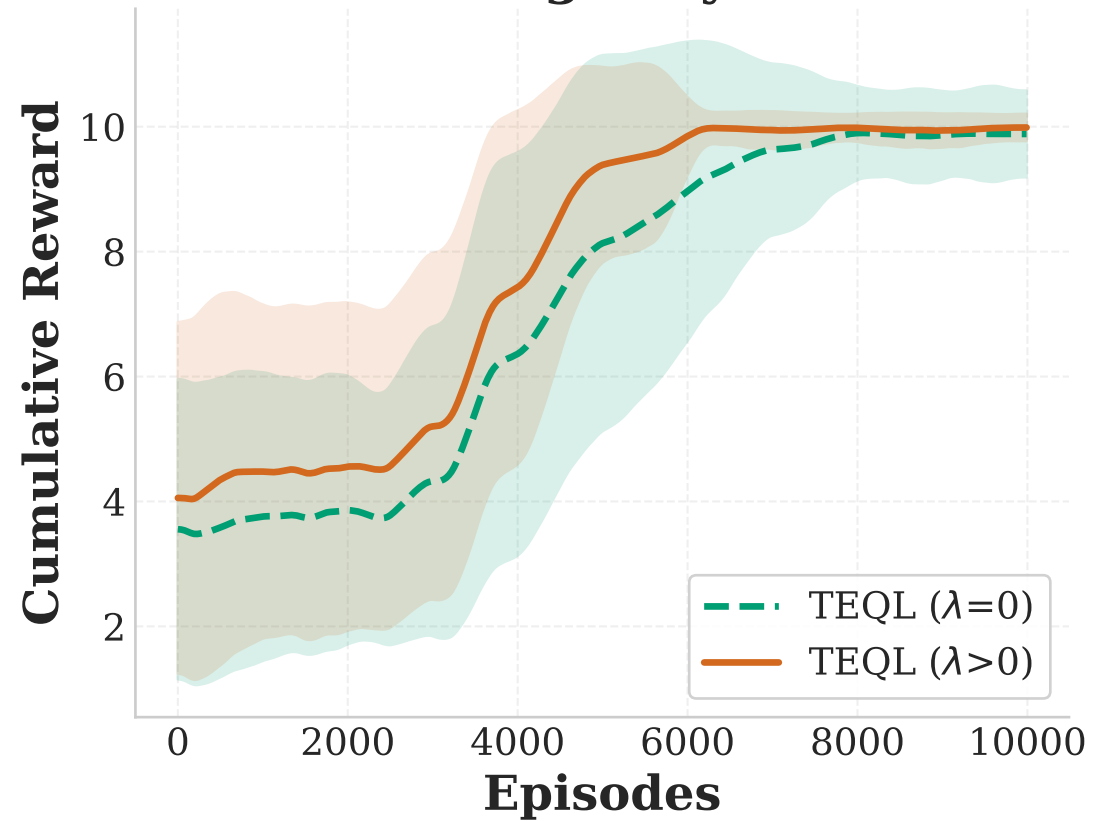
Highway
