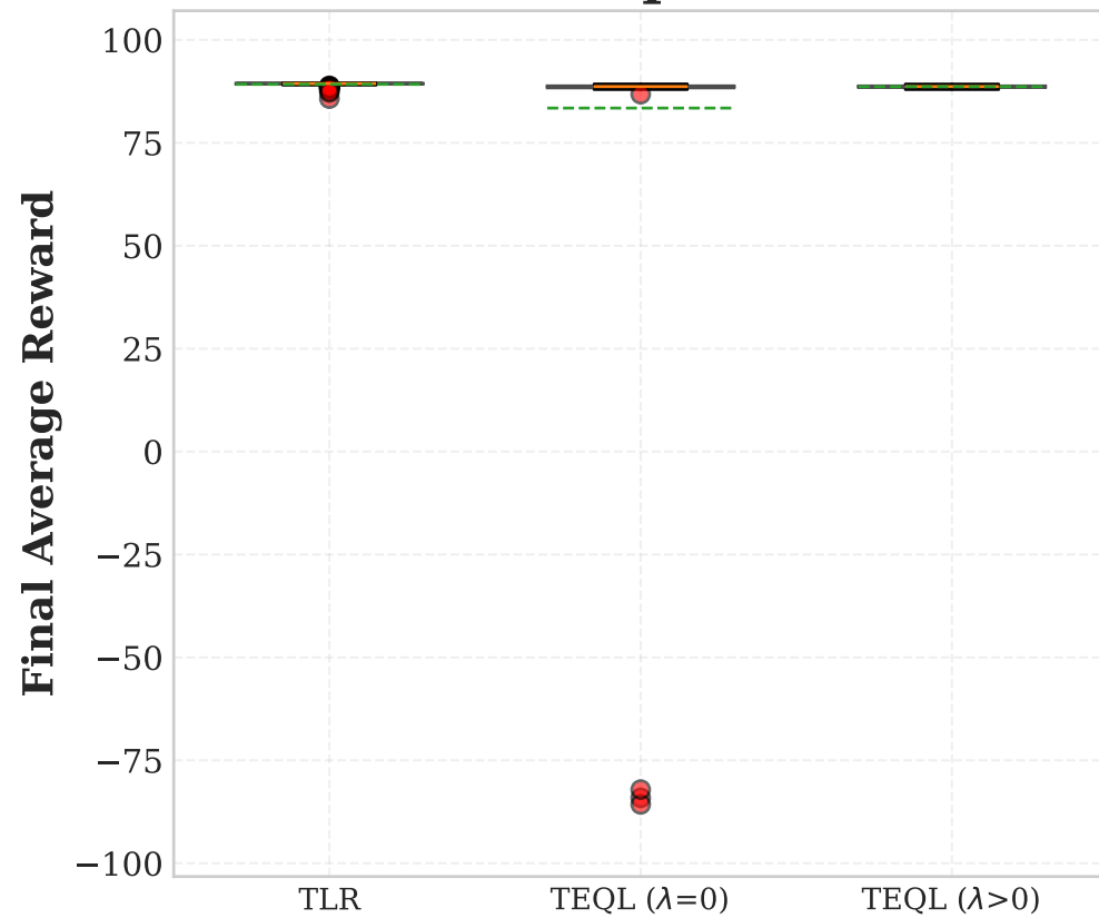
Cartpole
