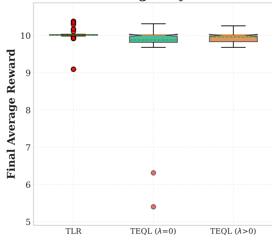
Highway
