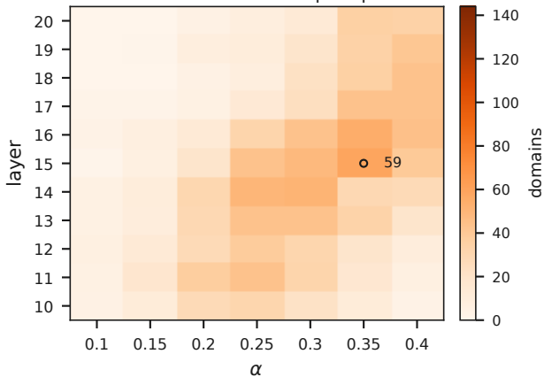
8B 10-word: CAA vs prompt
