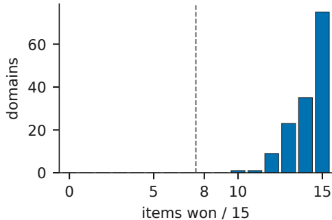
CAA vs silent 144/144 domains \geq 8/15
