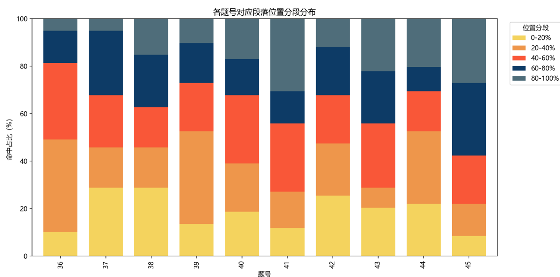
图 2: question_position_band_distribution.png
