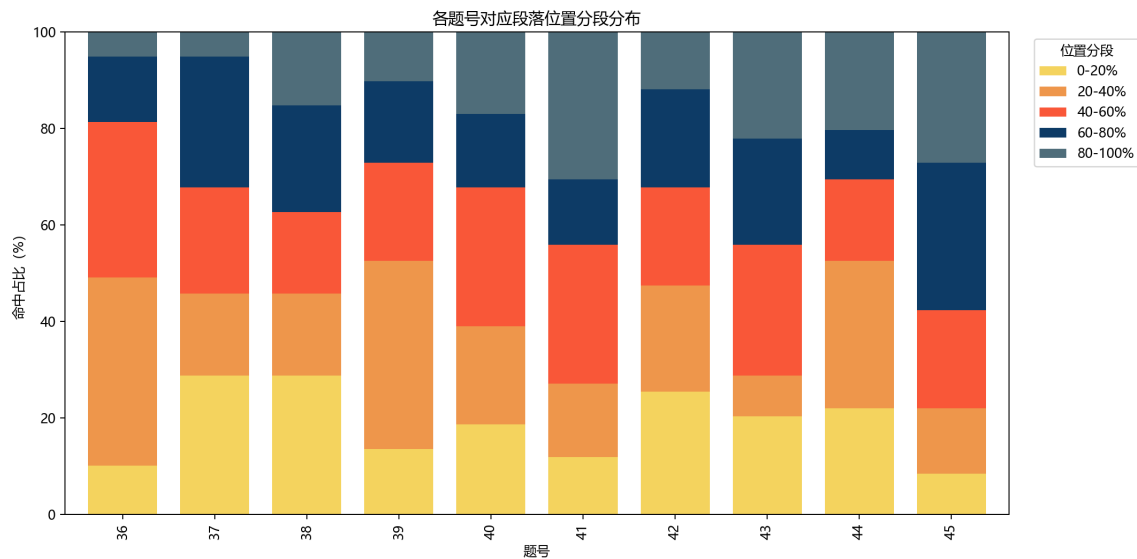
图 2: question_position_band_distribution.png
