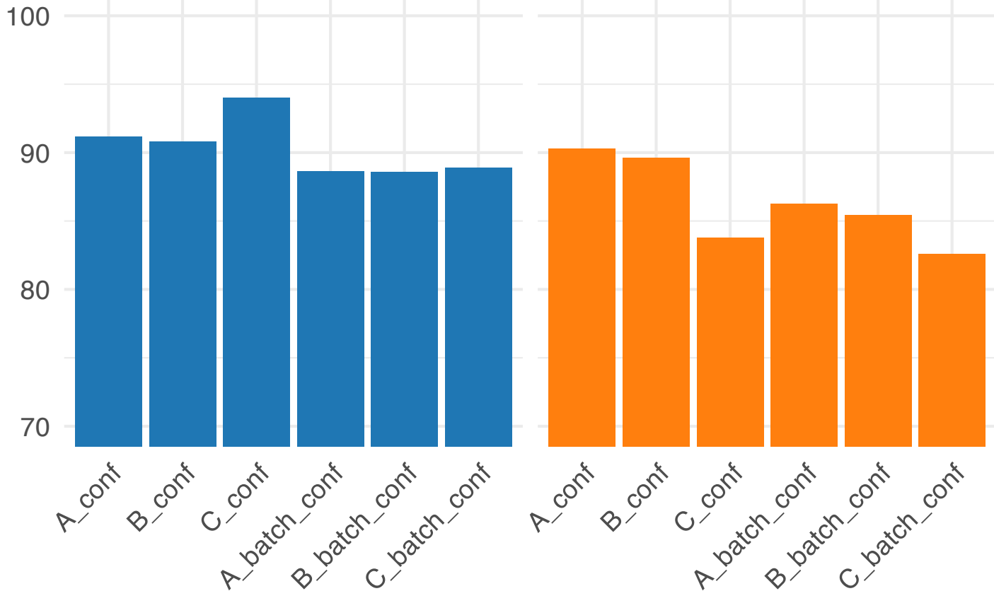
Mean LLM-reported Confidence
