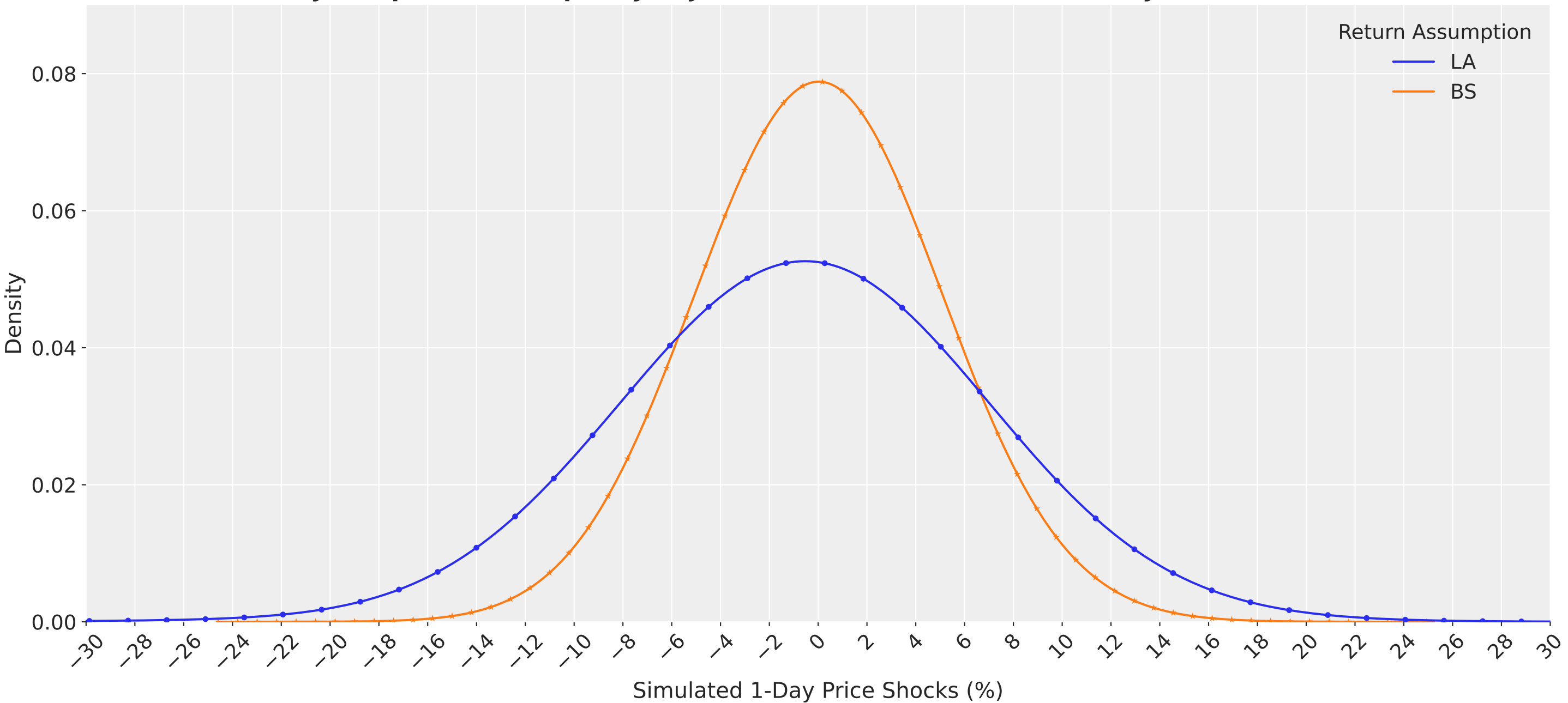
Density Comparison of Liquidity Adjusted (LA) and Baseline (BS) 1-Day Simulated Returns
